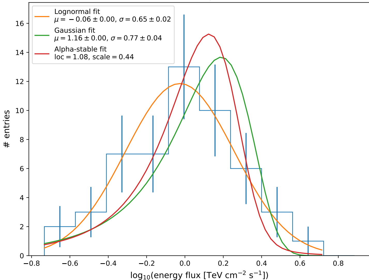
BLLac, cadence - 120 min 1 time per month - CTAO simulation
